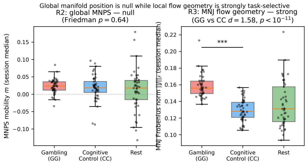
Figure 2: Global MNPS mobility ( m ) shows no reliable task separation (left), while MNJ Frobenius norm shows a large, robust GG > CC effect (right). Points are session medians; boxes show quartiles across N = 44-45 subjects.
