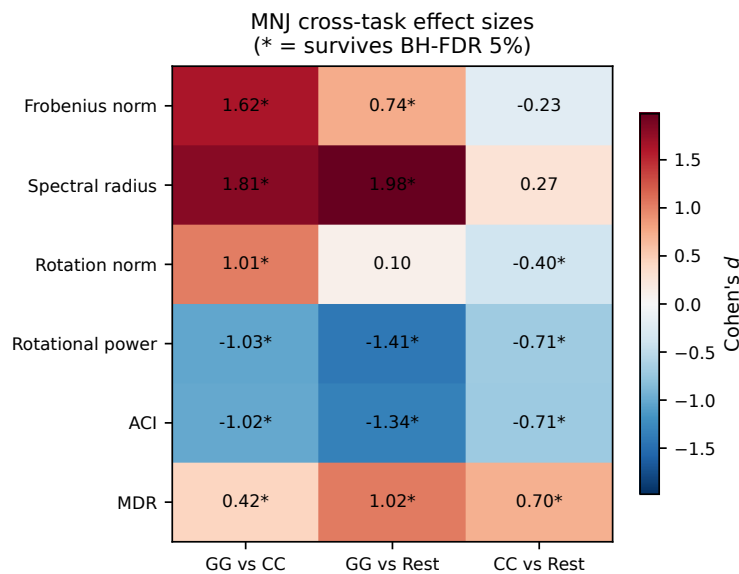
Figure 3: Cohen’s d for all six MNJ metrics across the three pairwise task contrasts. Asterisks mark contrasts surviving BH-FDR 5%. Gambling shows elevated absolute deformation (Frobenius, spectral radius) but reduced rotational structure (rotational power, ACI) relative to cognitive control and rest.
